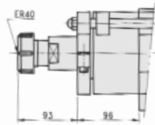
FD7-150-ER40
