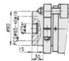
FD8-150-FB30
