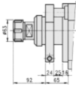
FD75-100-ER40
