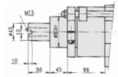
FD7-150-MT3B Multi
