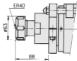
FD8-150-ER40
