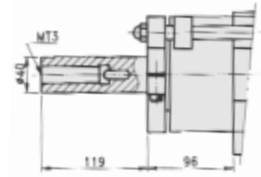
FD7-150-MT3A
