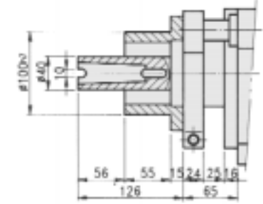
FD75-100-MT3A Multi
