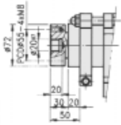
F7N-80-FB20
